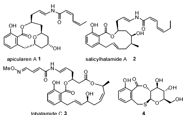
Figure 1. Structures 1–4.
