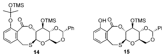
Figure 2. Silylated lactones 14 and 15 .
